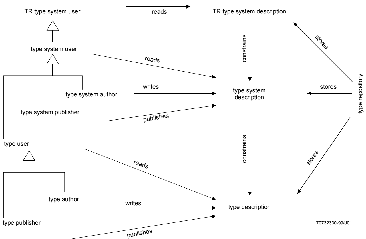
Figure 1 – Roles and Activities in the Type Repository Community
