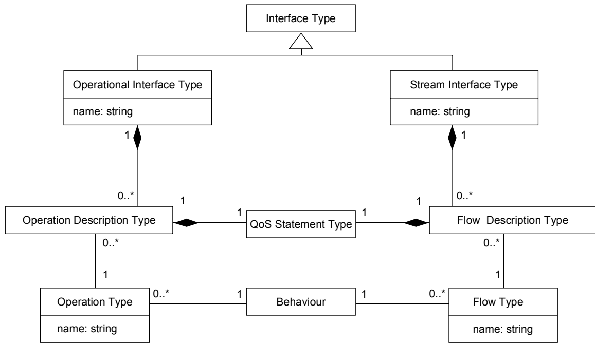
Figure A.7 – Interface Types for Binding
