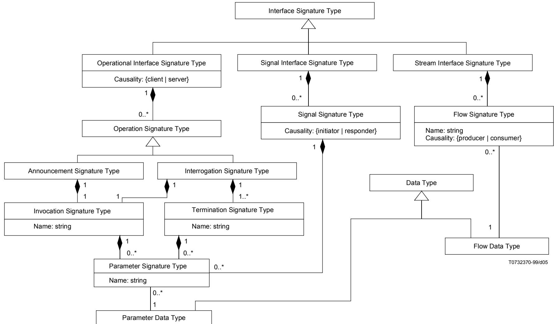
Figure A.4 – Interface Signature Types and Data Types
